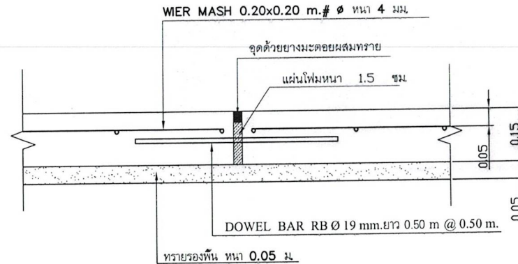
EXPANSION JOINT
