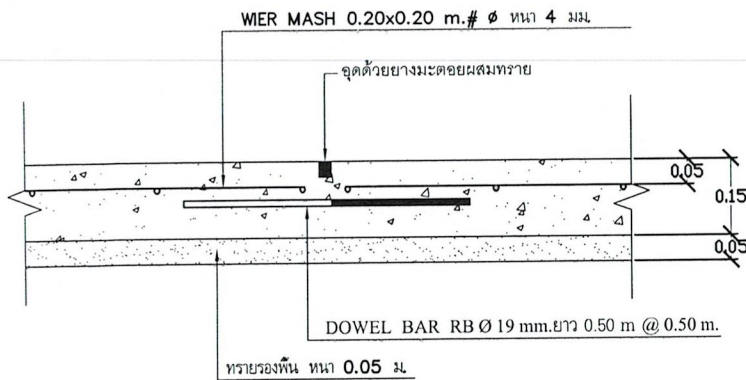
CONTRACTION JOINT
