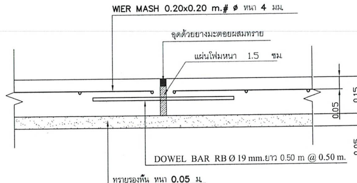
EXPANSION JOINT Scale : 100
