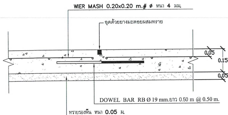
CONTRACTION JOINT Scale : 100
