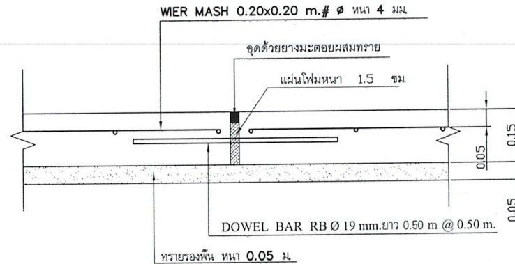
EXPANSION JOINT
